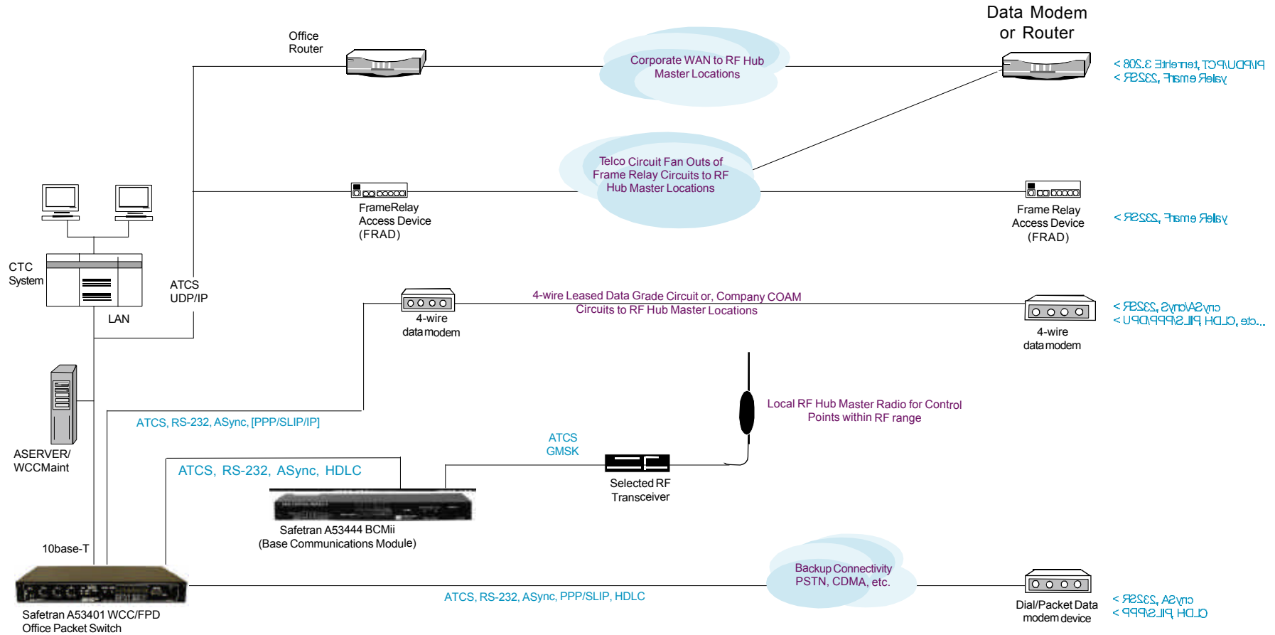
FIGURE II – FIELD CODE NETWORK OFFICE SYSTEM INTERFACE OFFICE CONNECTIVITY OPTIONS
