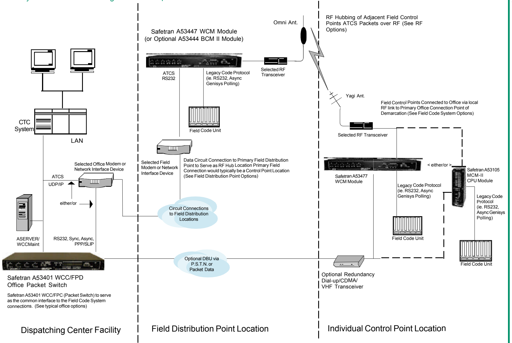
CTC system overview illustrating the three components of CTC train control architecture and the three Field Code Network interface considerations
